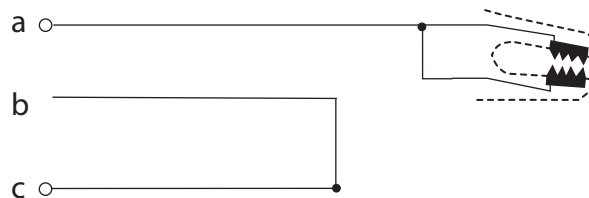
Fig. 7: Type 70HK connecting cable 3 x 1.5 mm 2
